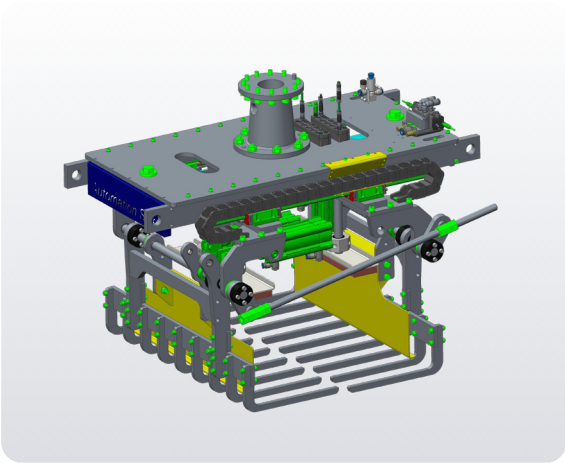
Bag Gripper
