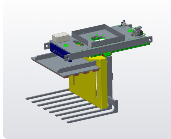
Sliding Fork Gripper
