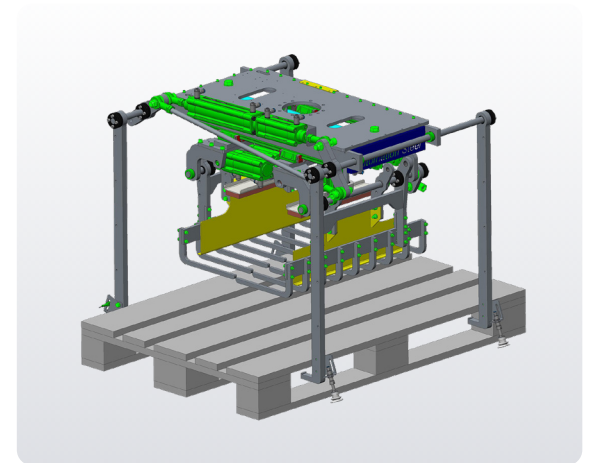
Bag & Pallet Gripper
